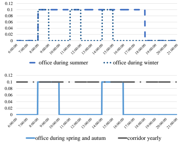
Figure 5: Window opening strategies for the “Historical building”
