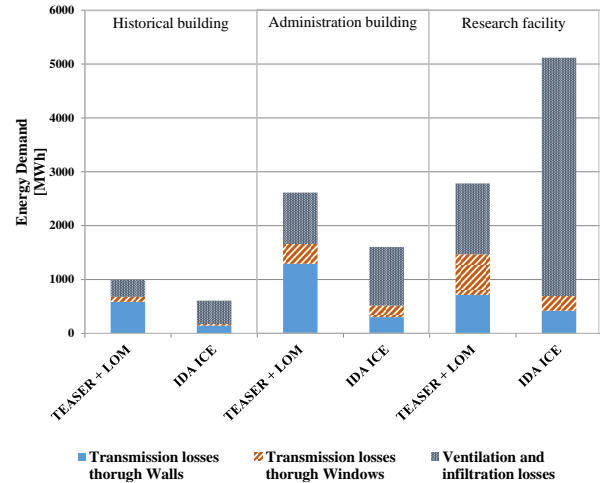
Figure 7: Distribution of heat losses (transmission through wall and window, ventilation) for each building; estimated with TEASER and LOM and IDA ICE
