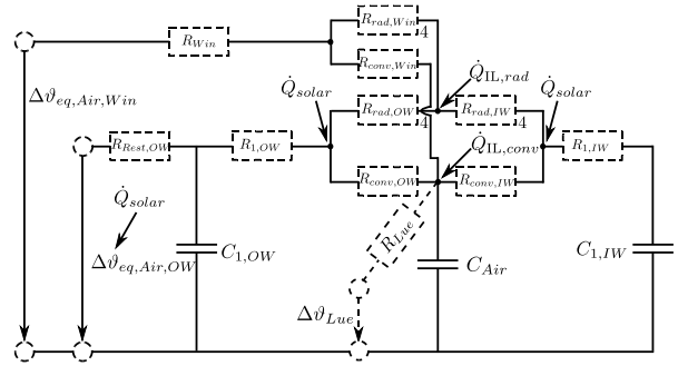
Figure 1: Low Order Model (Lauster 2014).
