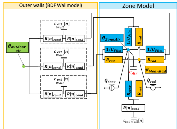
Figure 2: Network model of the IDA ICE 4.7 “CeSimZone”-model.
