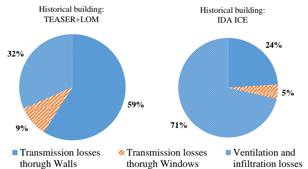
Figure 8: Allocation of losses (transmission through wall and window, ventilation) for the “Historical building” estimated with TEASER, LOM and IDA ICE
