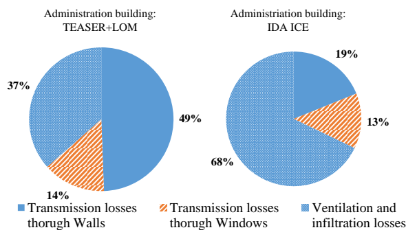
Figure 9: Allocation of losses (transmission through wall and window, ventilation) for the “Administration building” estimated with TEASER, LOM and IDA ICE
